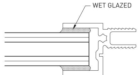
14mm I.G.U. ADAPTOR
