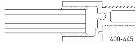
10mm GLASS ADAPTOR
